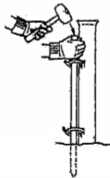
Fig. 4: Insert white oak stake into the two ties and drive into the ground until the top of the stake is 2-3" above the top tie.
